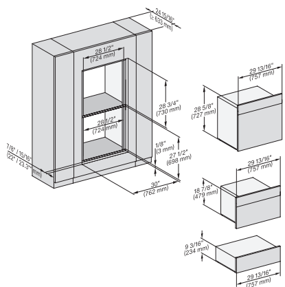
H 6x80 BP, H 6x70 BM, ESW 6x85, H 6x80-2BP, H2x80BP, H7x0BP/BM/BPX, ESW7x70, EVS7670 Flush inset, NA
