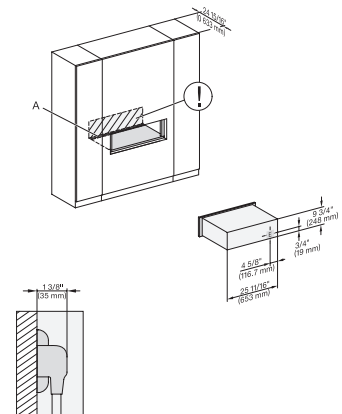
EVS7670, inset, 30 Zoll, Flush – NA
