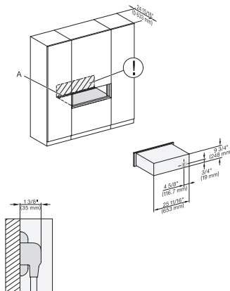
EVS7670, inset, 30 Zoll, Flush – NA
