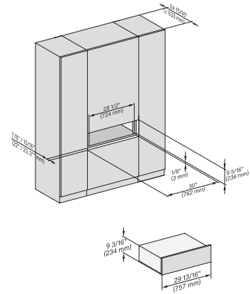
EVS7670, inset, 30 Zoll, Flush – NA
