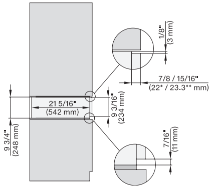
EVS7670, side view, 30 Zoll, Flush – NA
