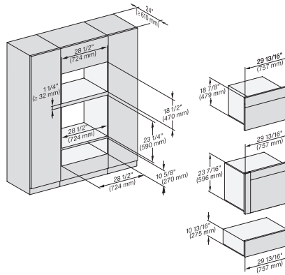
(H6560B, H6x60BP, DGC686xAM)+EBA680B; H6x70BM, ESW6x80, DGC676x, NA7000 Fitting Combi, Installation drawing, Proud, NA
