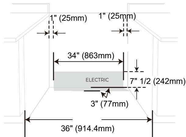
UTILITY LOCATIONS
