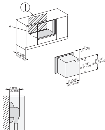
A – Cut-out (4" x 28" / 100 mm x 720 mm) in the bottom of the cabinet for power cord and ventilation, – Electrical and water supplies are recommended to be placed in adjacent cabinetry., Additional cabinet depth is required when placing the electrical and water supplies behind the appliance., E = Electric connection,
