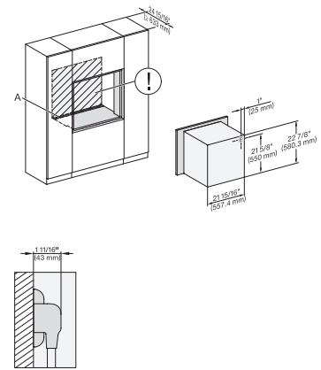
A – Cut-out (4" x 28" / 100 mm x 720 mm) in the bottom of the cabinet for power cord and ventilation, – Electrical and water supplies are recommended to be placed in adjacent cabinetry., Additional cabinet depth is required when placing the Electrical and water supplies behind the appliance., E = Electric connection
