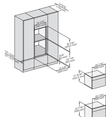
DGC7x4x, H7x40BM, H7x6xBP, Einbau, 30 Zoll Flush inset, combi, 650S, 450S
