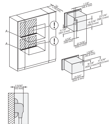
DGC786x(+EBA7848), H7x40BM(+EBA7848), Installation, 30 Zoll, Proud, combi, wide front, XXL, 450S
