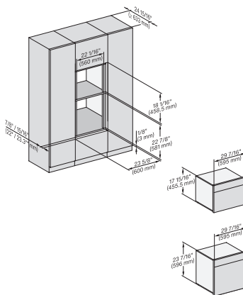
DGC7x4x, H7x40BM, H7x6x, H7x6xBP, Einbau, 30 Zoll Flush inset, combi, 650S, 450S
