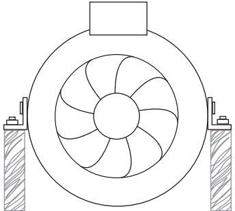
Horizontal Installation with out Kit
