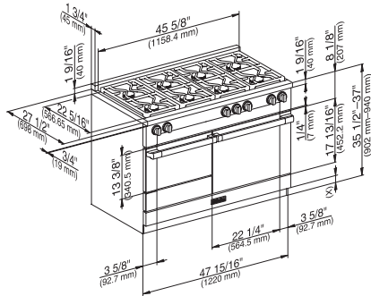
HR1954G, HR1954-2, HR1954-3 (installation drawing)
