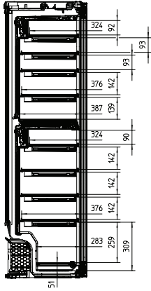
KWT6722iS, Interior dimensions (Installation drawings)
