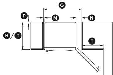
Flush with refrigerator door – full door rotation
