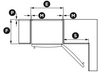
Flush with refrigerator chassis – full door rotation
