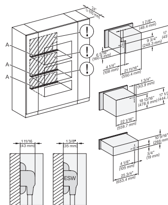
DGC7x4x+EBA7848, H7x70BM(X), ESW7x80, Installation, 30 Zoll. Proud. combi. wide front. XL
