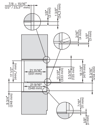
H 6x70 BM, ESW 6x85, H7x70, EVS 7670 Combi, installation drawing, Flush inset, NA
