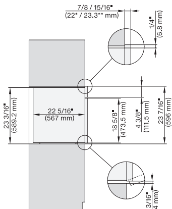
DGC 6x6x (AM) + EBA 6808, DGC 786x (+EBA 7868) side view, installation drawing, Proud, NA
