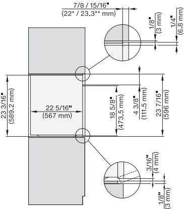
DGC 6x6x (AM) + EBA 6808, DGC 786x (EBA 7868) side view, installation drawing, Flush inset, NA
